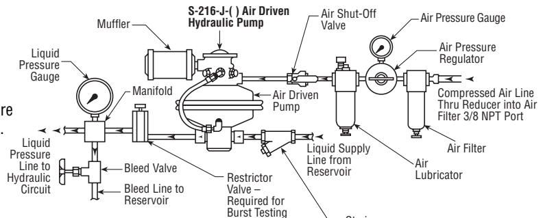
PUMP AND ACCESSORIES — TYPICAL ARRANGEMENT
