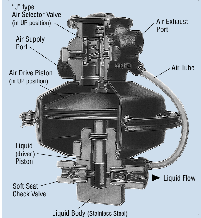
PUMP AIR PISTON IN UP POSITION
